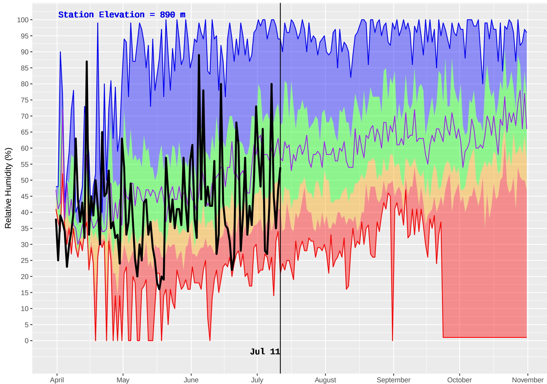
ISKUT (112) : Historical (1979–2016) and Current (2018) Noon Relative Humidity
