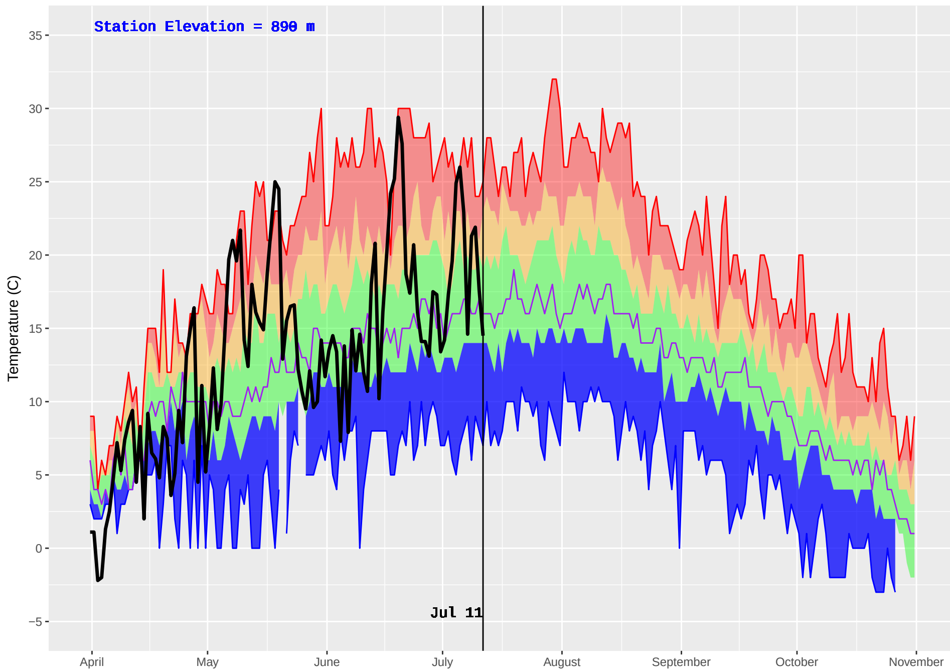
ISKUT (112) : Historical (1979–2016) and Current (2018) Noon Temperature
