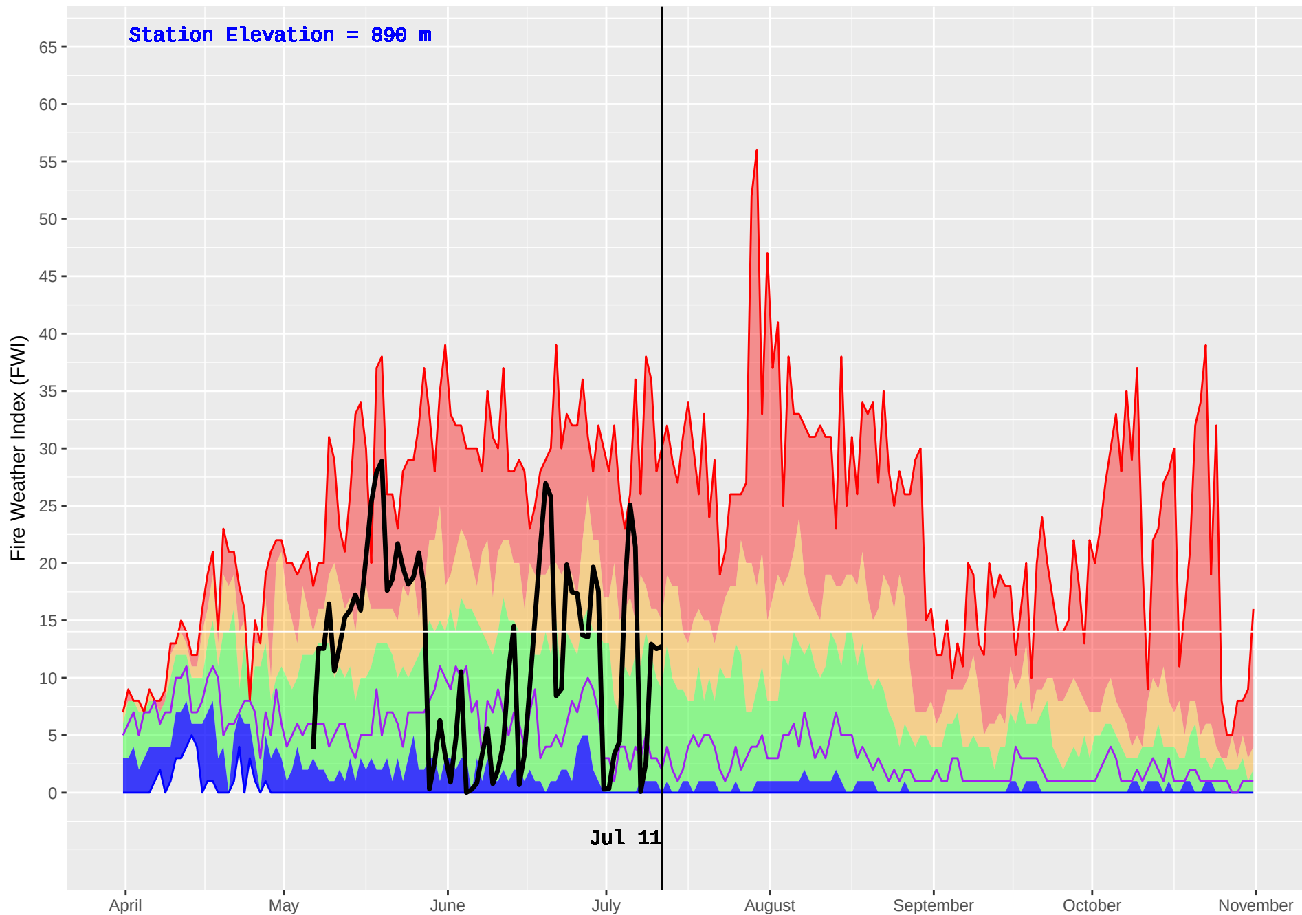
ISKUT (112) : Historical (1979–2016) and Current (2018) Noon Fire Weather Index (FWI)
